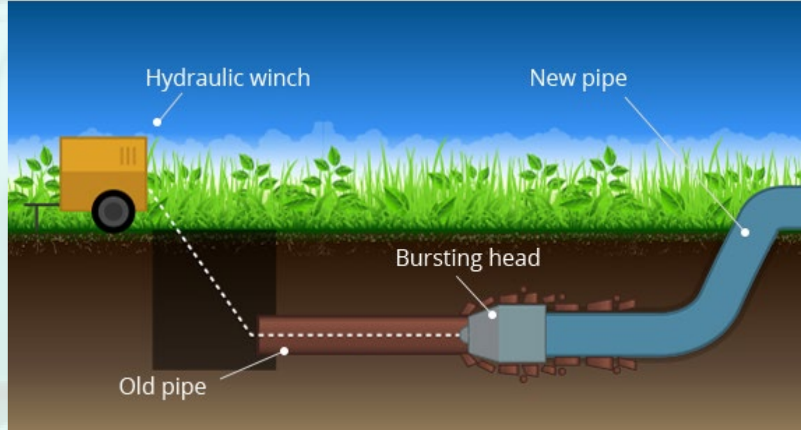
Pipe Bursting
